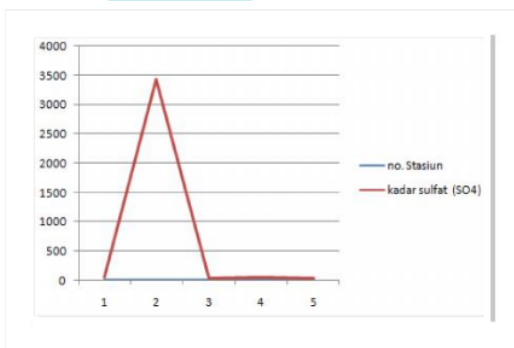
Figure 5. Sulfate Contamination (SO 4 ) at leachate sample
