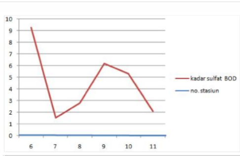
Figure 8. Contamination of BOD at water sample that produced by well
