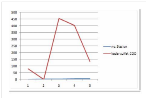
Figure 9. Contamination of COD at leachate sample.
