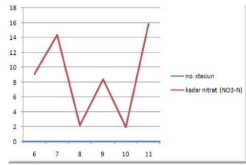
Figure 4. Nitrate Contamination ( \text{NO}_3\text{-N} ) at water sample that produced by well
