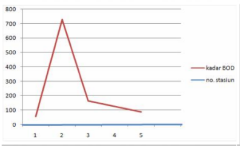
Figure 7. Contamination of BOD at leachate sample
