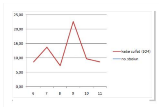
Figure 6. Sulfate Contamination (SO 4 ) at water sample that produced by well.
