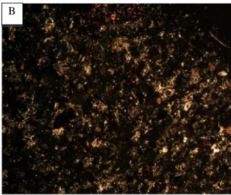
Figure 2. Outcrop view of coarse-grained tuff with colour light grey to yellow (a) and microphotograph view showing the mineral constituent (b).
