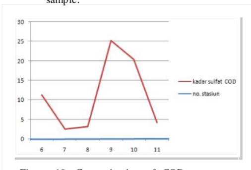
Figure 10. Contamination of COD at water sample that produced by well.
