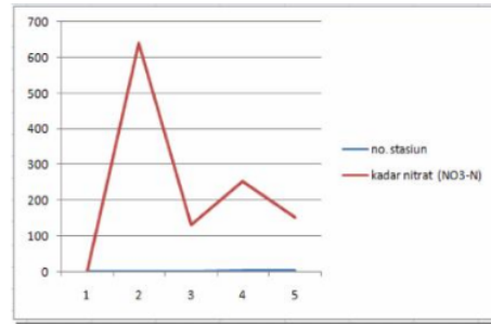
Figure 3. Nitrate Contamination ( \text{NO}_3\text{-N} ) at leachate sample
