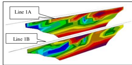
Figure 11. Geoelectric Inversion Section of resistivity line 1A and 1B
